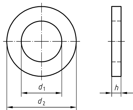
Figure 1 — Dimensions
