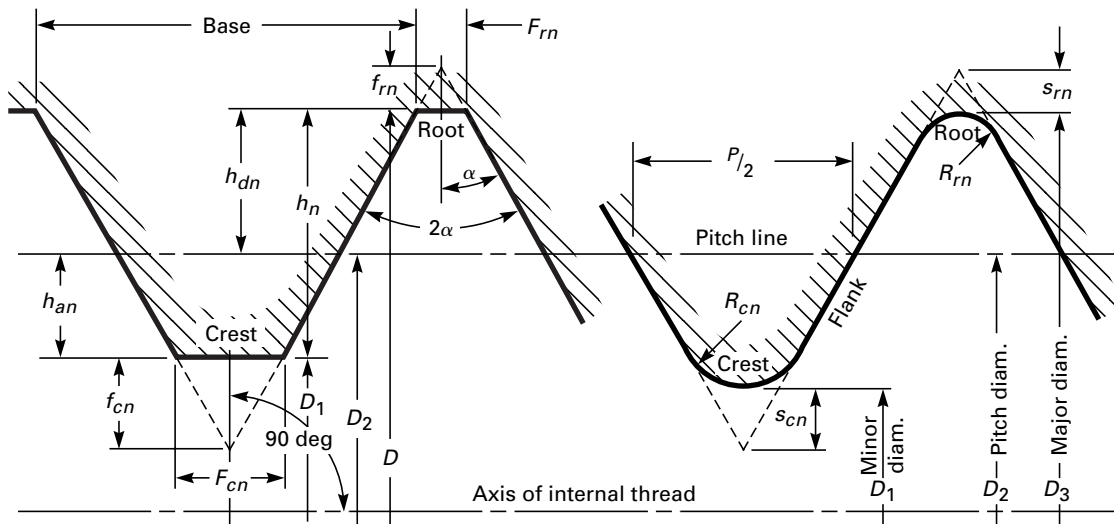
Internal Thread
