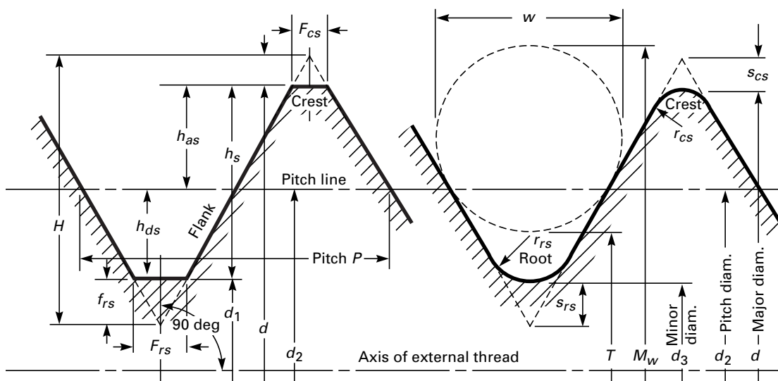
External Thread
